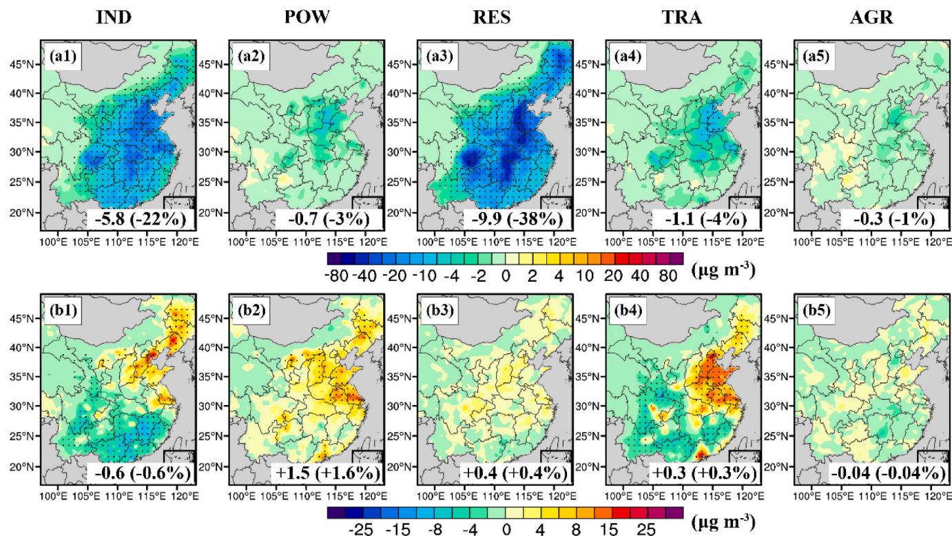
Fig. 2. Spatial distribution of changed PM 2.5 (upper) and MDA8 O 3 (bottom) concentrations due to future anthropogenic emission reductions by each sector of industry (IND, a1-b1), thermal power (POW, a2-b2), residential (RES, a3-b3), transportation (TRA, a4-b4), and agriculture (AGR, a5-b5) relative to that in 2018. Dotted areas indicate grid cells where the concentration differences pass the 90% significance level based on a student t-test. The mean change averaged over the whole domain is also shown in the bottom right corner of each panel.
