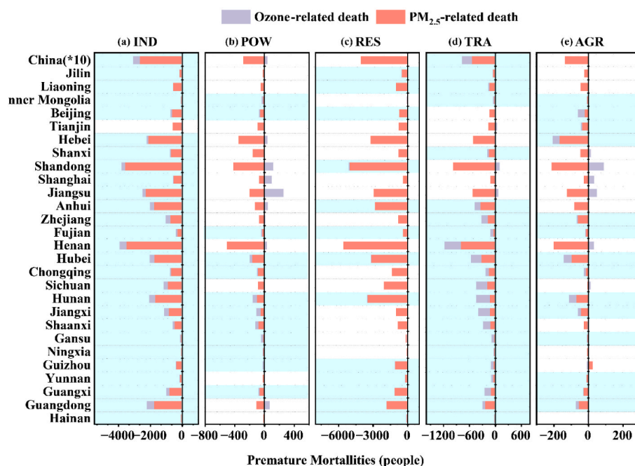
Fig. 4. Changes in premature deaths associated with short-term exposure to \text{PM}_{2.5} and \text{MDA8 O}_3 for each province in China due to reductions in anthropogenic emission by sectors of industry (IND, a), thermal power (POW, b), residential (RES, c), transportation (TRA, d), and agriculture (AGR, e) from 2018 to 2060. Purple (red) bar means changes in ozone-related ( \text{PM}_{2.5} -related) premature deaths. The light cyan backgrounds indicate synergistic improvement in health burden, which mean both ozone-related and \text{PM}_{2.5} -related premature deaths are decreased. (For interpretation of the references to colour in this figure legend, the reader is referred to the Web version of this article.)
