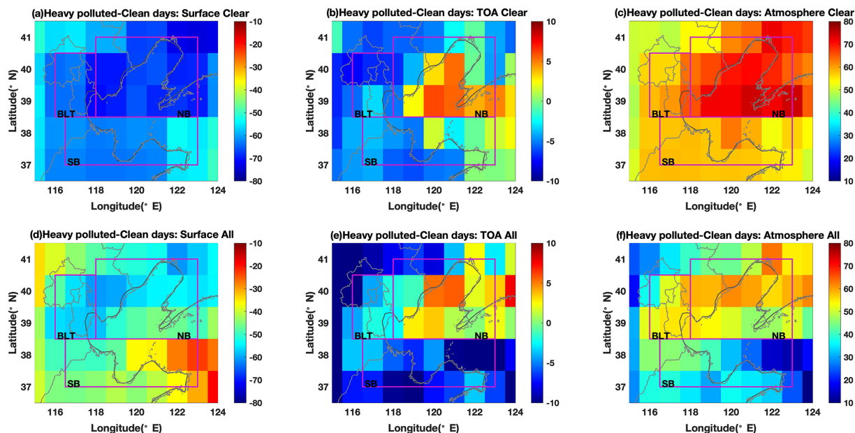
Figure 4. The short-wave radiative forcing ( \text{Wm}^{-2} ) on regional PM 2.5 heavy pollution days calculated from the difference between CERES net radiative fluxes on regional heavy pollution days and the mean of clean days for all stations: (a, d) at the surface; (b, e) at the top of atmosphere (TOA); (c, f) in the atmosphere, in clear sky (a–c) and all sky (d–f) .
